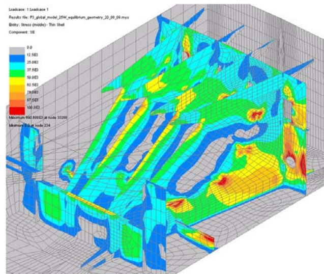
Fig. 7: Stresses in cable anchorage plates.
