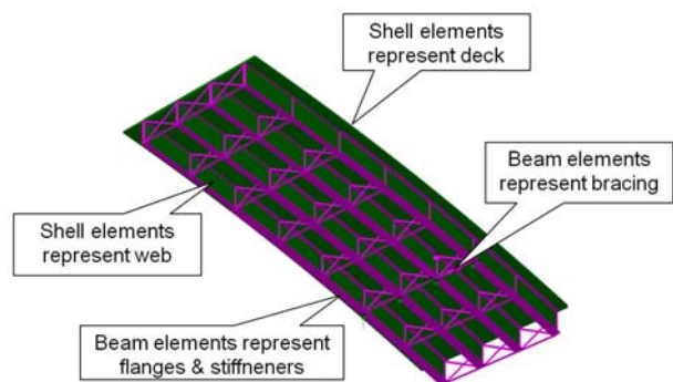
Fig. 5: Mixed beam and shell element modelling.
