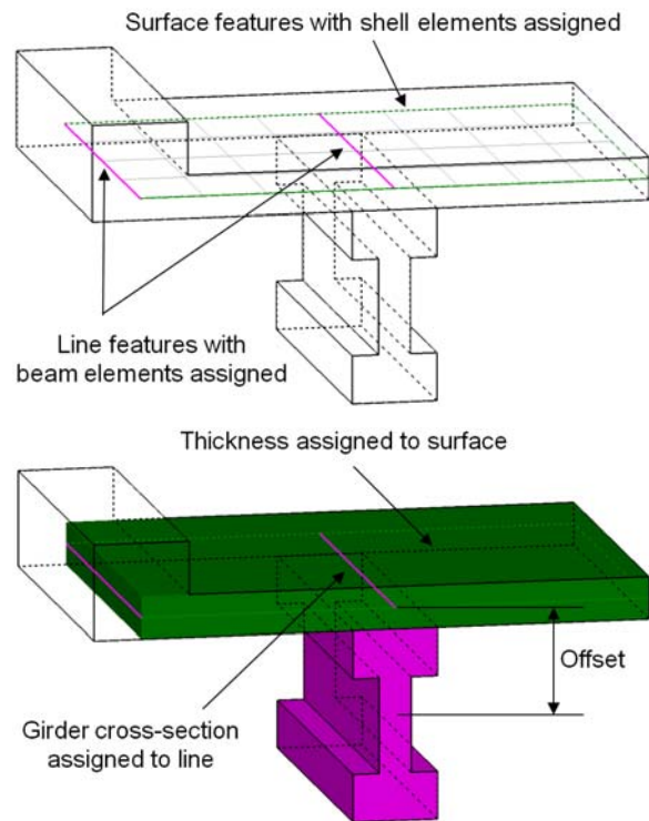
Fig. 4: Shell-on beam model, showing offset for main girder (where in-plane loads are not applicable)
