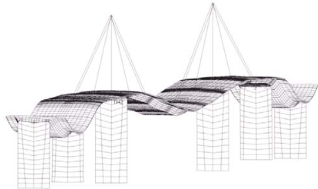
Fig. 6: Shell and beam model of West Gate Bridge, showing exaggerated permanent load deflection and cable creep.
