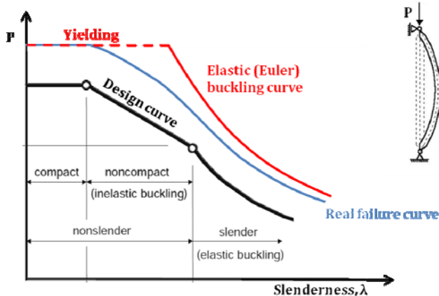
Fig. 8: Theoretical, real and codified buckling curves.
