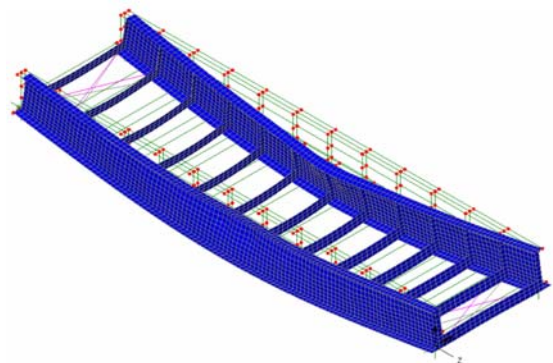
Fig. 2: Half-through girder modelling
