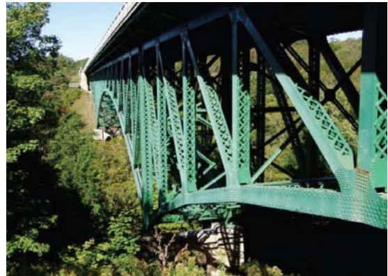
Fig. 1: Cut River Bridge.
